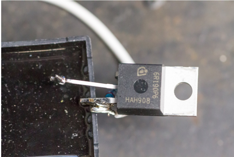
Figure 6: MOSFET Drain on bottom, Source in middle, and Gate on top
