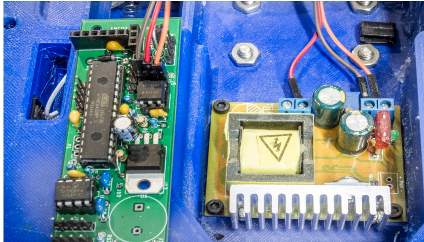
Figure 17: Connecting High-Voltage Boost Converter to Control Board
