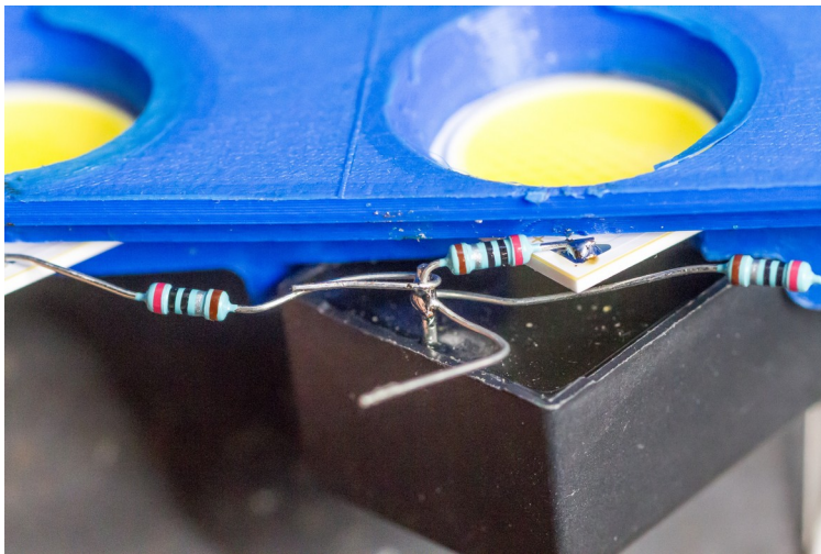
Figure 11: Careful routing of resistor leads
