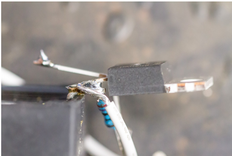
Figure 7: Ground wire soldered to MOSFET Source / Capacitor cathode
