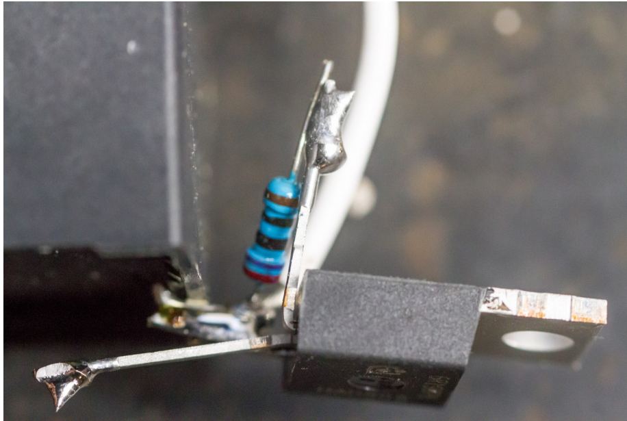
Figure 8: 1/4W resistor from MOSFET Gate to Source
