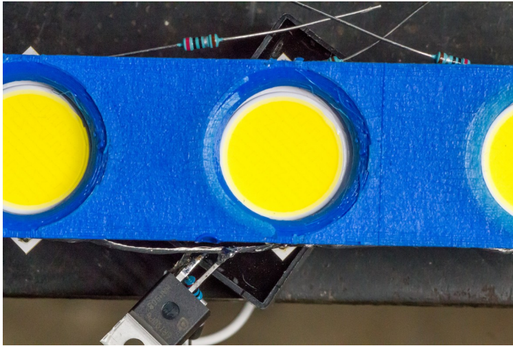
Figure 10: MOSFET Drain (middle) to LED cathode rail
