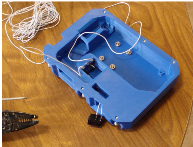
Figure 16: Wiring to power switch installed, proceed to slide power switch into case
