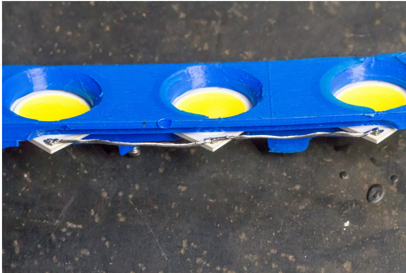
Figure 4: 22AWG wire soldered to LED cathodes (negative)
