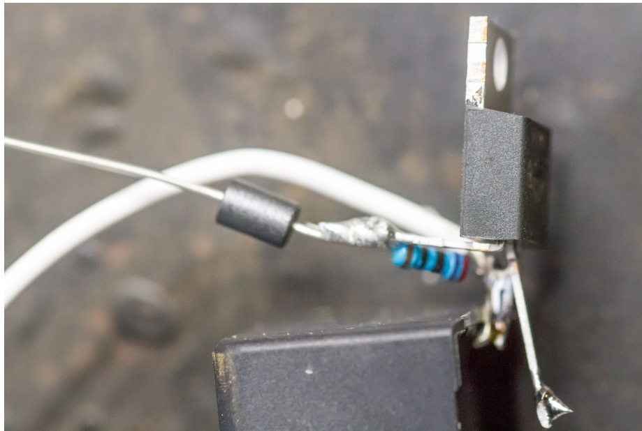
Figure 9: Short distance from ferrite bead to MOSFET
