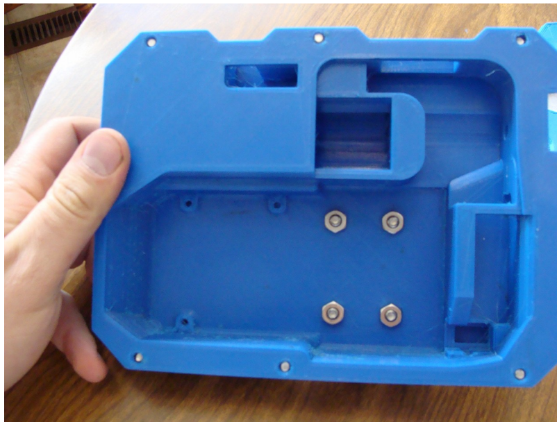
Figure 15: Case interior view, M5 nuts securing Arca-Swiss QR plate
