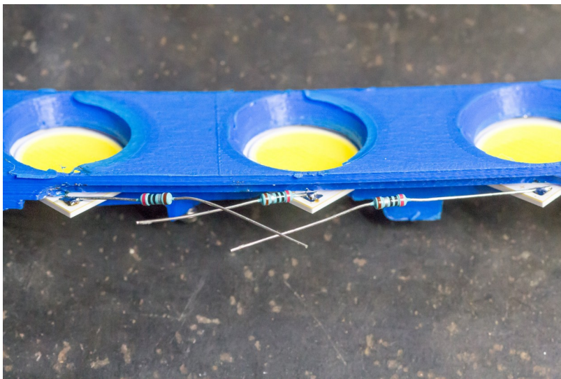
Figure 5: 2-ohm series resistors
